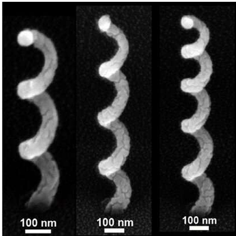
Helix nano-antennas. Nano-antennae were produced in an electron microscope by direct electron-beam writing. Created from Lyme spirochetes ( Borellia burgdorferi )? (Thanks to Ashley Noel, August 24, 2019.)
