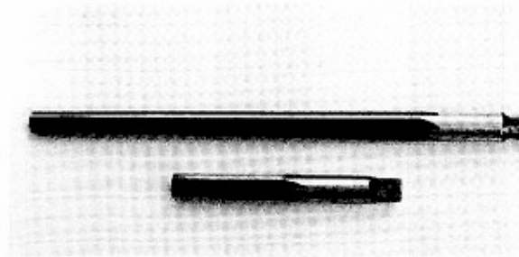
PHOTO 12: Taper pin reamer shown before and after cutting.
