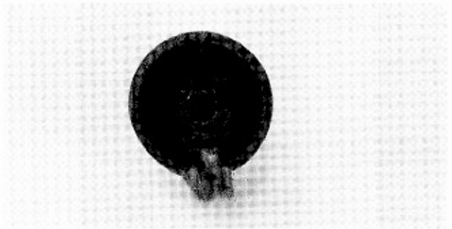
PHOTO 21: Firing pin rod fitted inside spring pin. The top of the rod should be 2.5 mm below the end of the spring pin.
