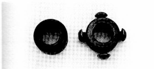
PHOTO 10: Steel collar shown alongside modified collar with four socket screws fitted.
