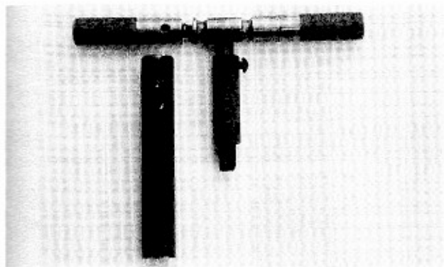
PHOTO 14: Complete reamer assembly. Sleeve is shown in position with reamer guide alongside.
