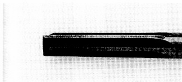
PHOTO 13: Side view of finished reamer. The top flute has been sharpened while the lower flute has been removed.
