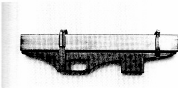
PHOTO 6: Upper and lower receivers clamped together with two hose clips.
