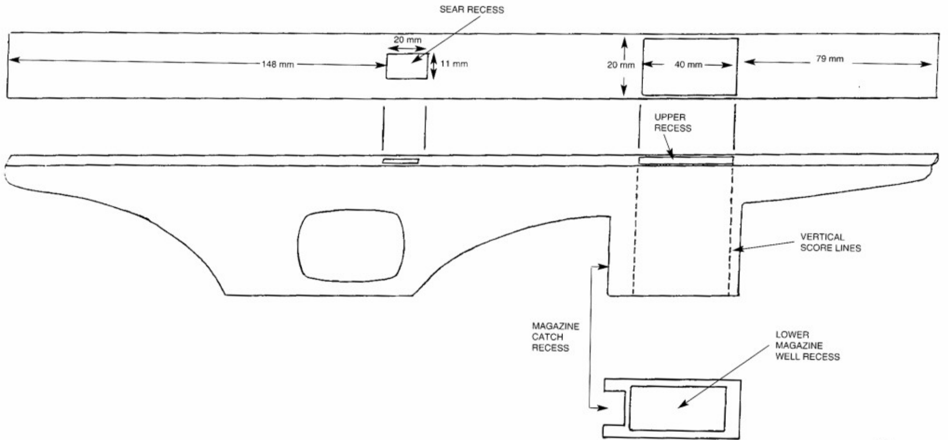
FIGURE C RECESS POSITIONS
