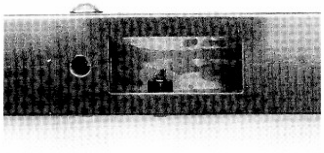
PHOTO 28: The ejector fitted to the receiver as seen through the magazine well recess.
