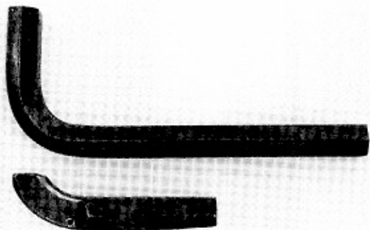
PHOTO 40: The sear before and after modification. Note the position of the spring pin.
