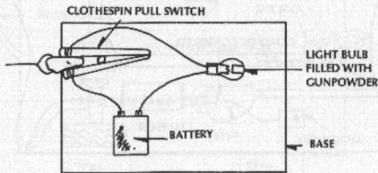
1. FIRING DEVICE
