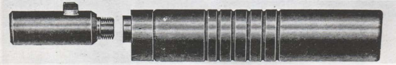
Examples of the clamps and couplers used to attach the original Maxim silencers to the weapons of the day. These couplings sold for $2.50, while the silencers themselves sold for $7.00.
