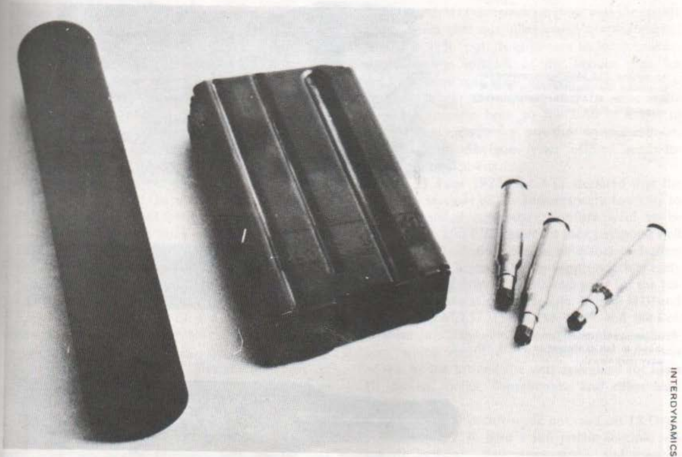
The Interdynamics suppressor, special magazine and the subsonic ammunition they sell as a total suppression system.
