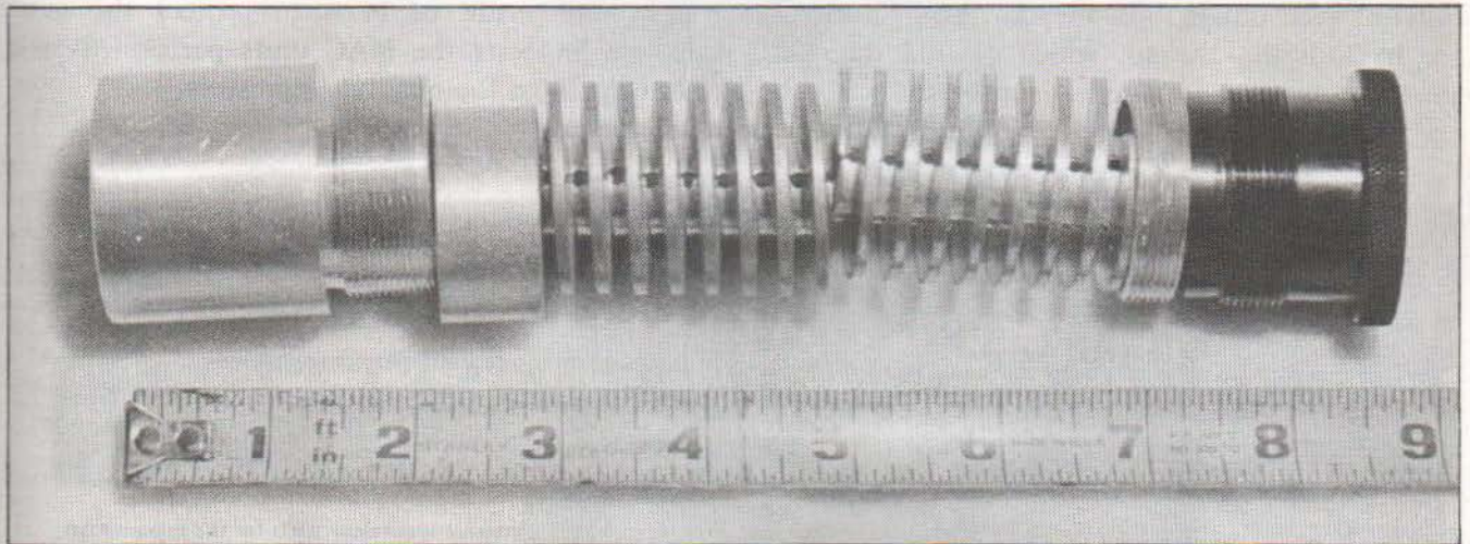
This is the standard R. F. P. mini kit using a MAC 10 outer tube. The unit is about nine inches long and will fit various weapons.
