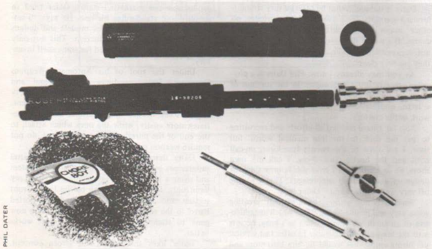
A totally disassembled RST suppressor with all parts, tools, and packing materials.
