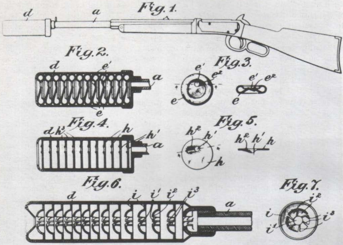
The patent illustration for H. P. Maxim's first truly successful silencer.
