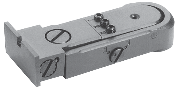
Les Baer PPC-Style Adjustable Rear Sight
